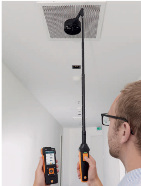
The 100 mm vane probe can be easily combined with the 90° angle and telescope, making measurements at ceiling outlets easier.
